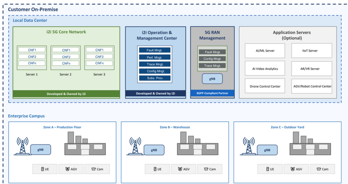
Figure 2: SNPN (On-Premise) Deployment — All 5G Core, RAN, and management components are hosted within the customer's local facility. Data remains fully on-premise, ensuring maximum sovereignty and security.
